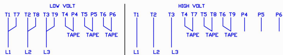
wiring diagram
