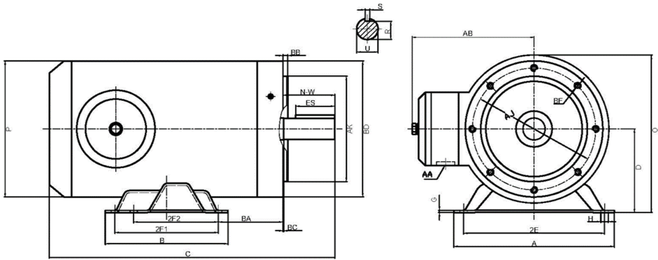
Dimensions in inches
